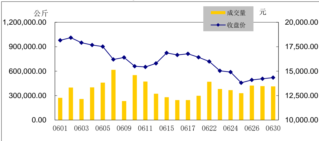
Ag(T+D)量价图
